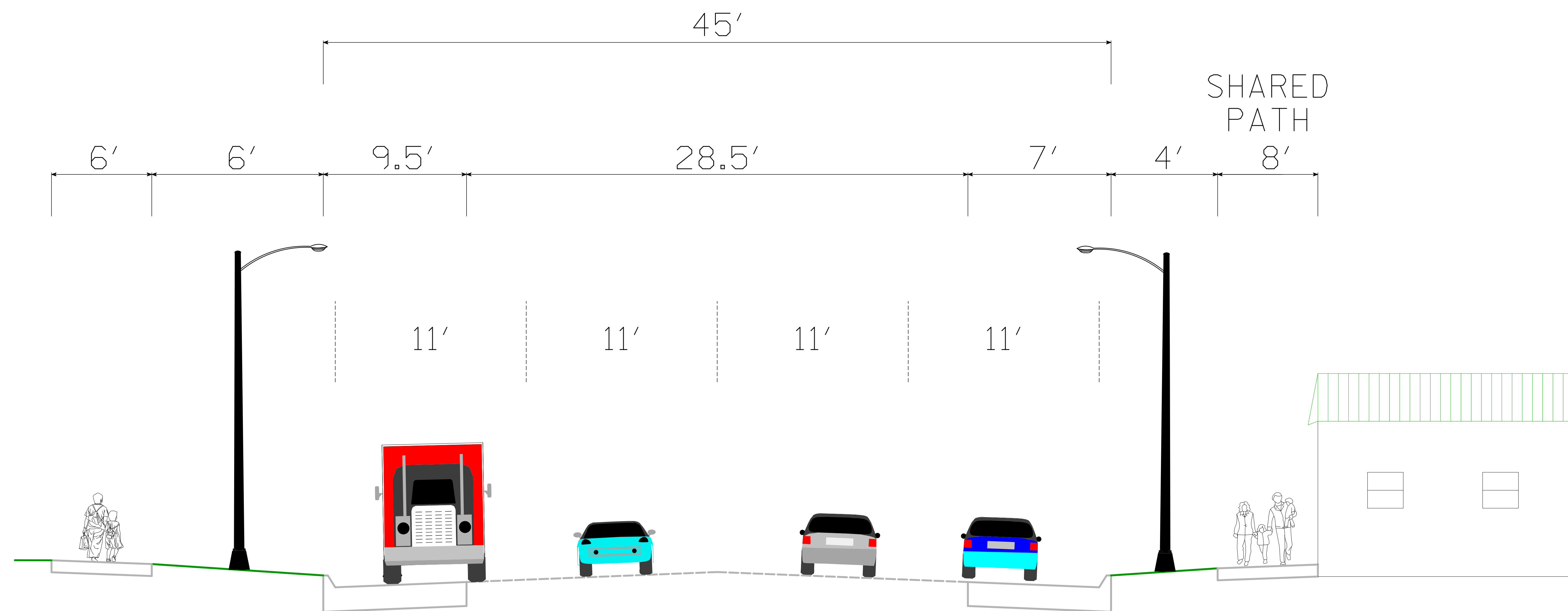
CROSS SECTION B 1st Avenue
