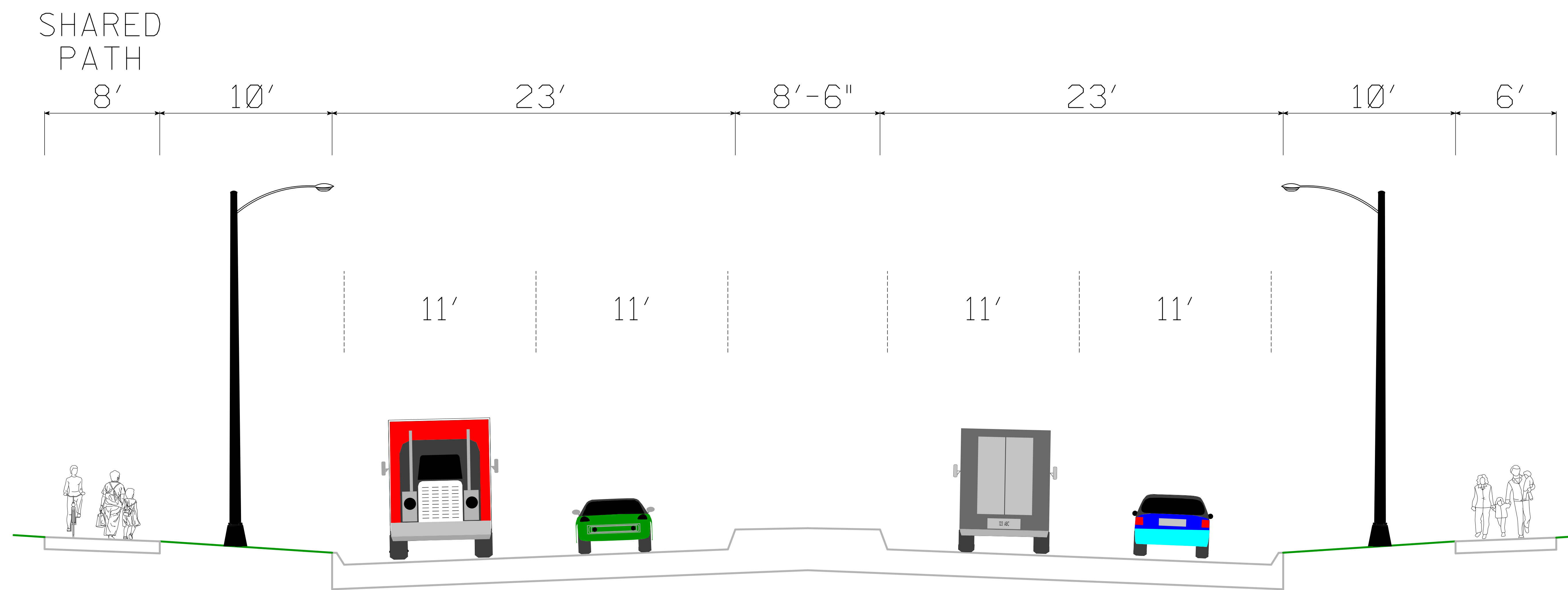
CROSS SECTION C 1st Avenue
