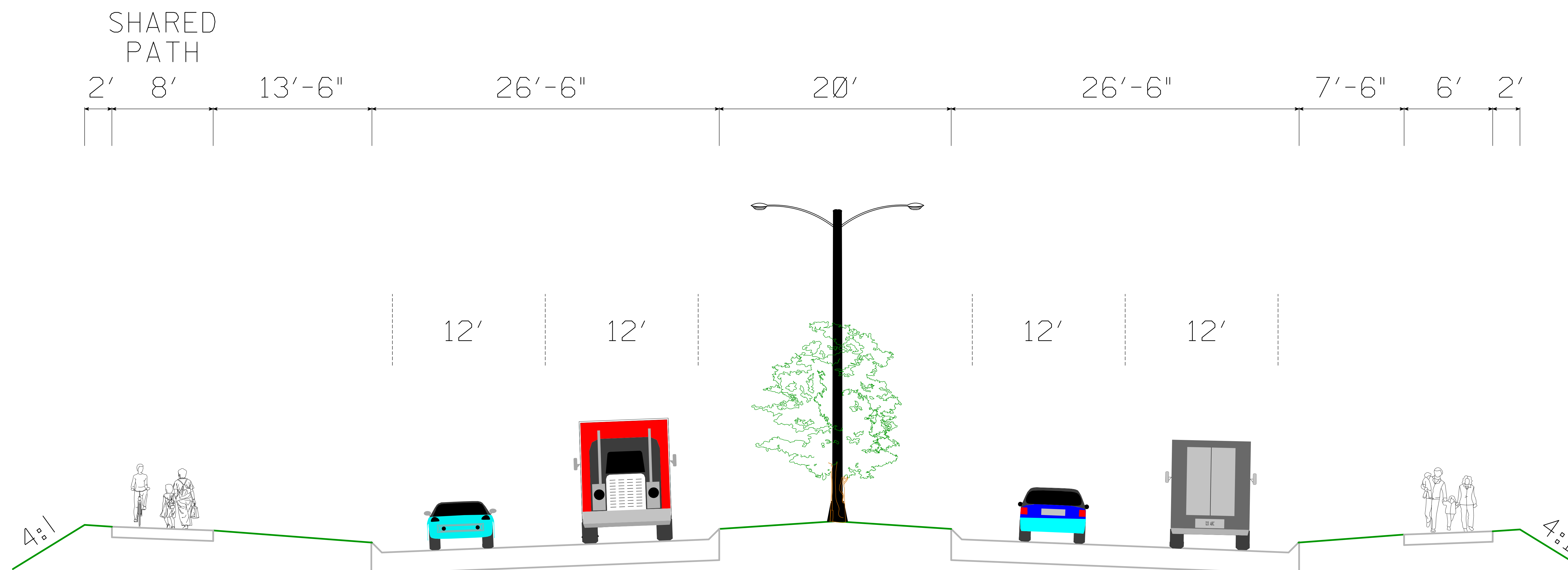
CROSS SECTION D 1st Avenue
